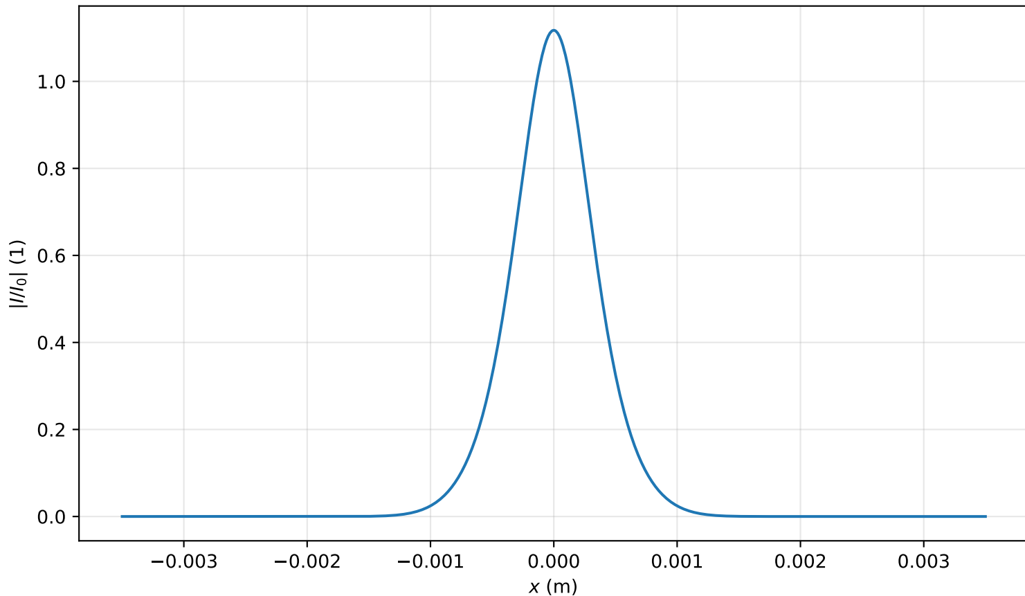
Intensity profile I(x, y = 0, z = 0.876m)/I_0 , P_{in}=0.6P_{cr} , artificial time
